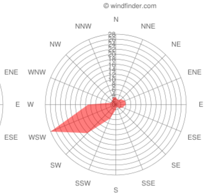
Wind dir. distribution Edinburgh Airport December
