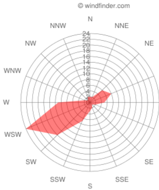
Wind dir. distribution Edinburgh Airport December
